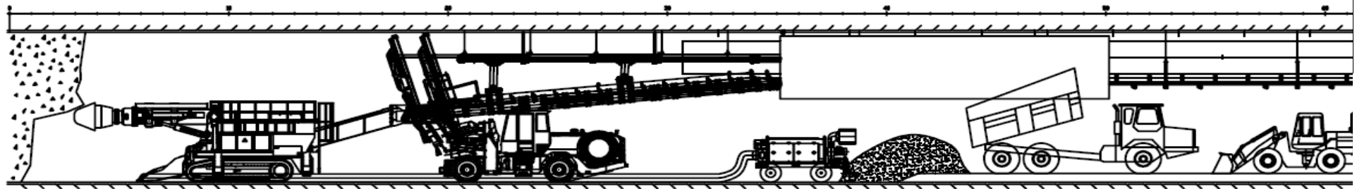
ROADHEADER CUTTING
