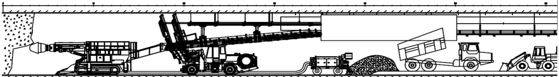
ROADHEADER CUTTING
